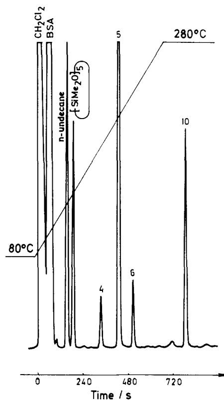
Figure 1. Gas chromatogram of the trimethylsilylated reaction mixture of \text{HO}[(\text{Me})_2\text{SiO}]_5\text{H} in \text{CH}_2\text{Cl}_2 in the presence of \text{CH}_3\text{SO}_3\text{H} at 35^\circ\text{C} taken at 30% of the substrate conversion. Initial concentrations of the substrate and the catalyst were 0.20 and 1.00 \times 10^{-4} \text{ mol}\cdot\text{dm}^{-3} , respectively. Unless denoted otherwise signals of trimethylsilylated linear oligomers \text{HO}[(\text{Me})_2\text{SiO}]_n\text{H} are denoted by n . Undecane is the internal standard and BSA is the silylating agent used in excess.
