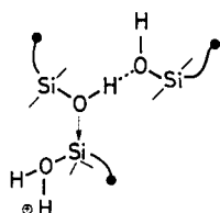
Scheme IV
