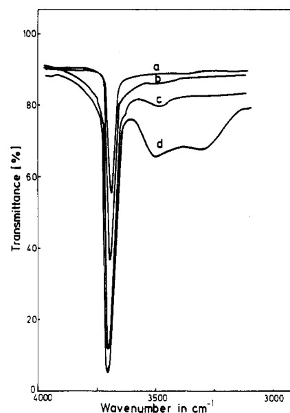
Figure 9. IR spectra of \text{Me}_3\text{SiOH} in \text{CCl}_4 at 35^\circ\text{C} . Concentrations in \text{mol}\cdot\text{dm}^{-3} are (a) 0.0080; (b) 0.0200; (c) 0.050; (d) 0.100. Path length, 2 mm.
