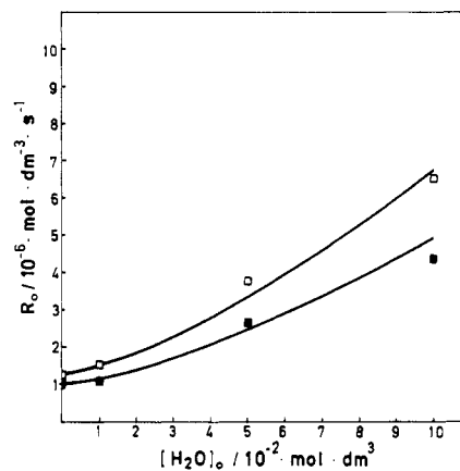
Figure 5. Effect of water initially introduced into the system on rates of product formation in the condensation of 0.10 \text{ mol} \cdot \text{dm}^{-3} \text{HO}[(\text{Me})_2\text{SiO}]_5\text{H} in methylene chloride with 1.00 \times 10^{-4} \text{ mol} \cdot \text{dm}^{-3} \text{CH}_3\text{SO}_3\text{H} at 35^\circ\text{C} : (□) [(\text{Me})_2\text{SiO}]_5 ; (■) \text{HO}[(\text{Me})_2\text{SiO}]_{10}\text{H} .
